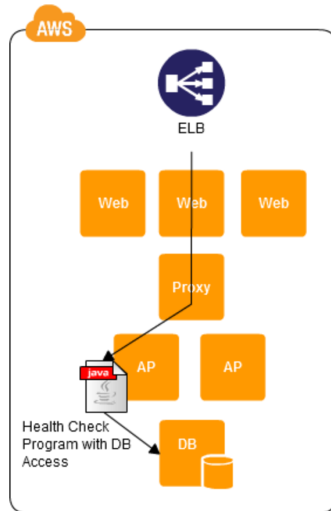
Deep Health Check Pattern
