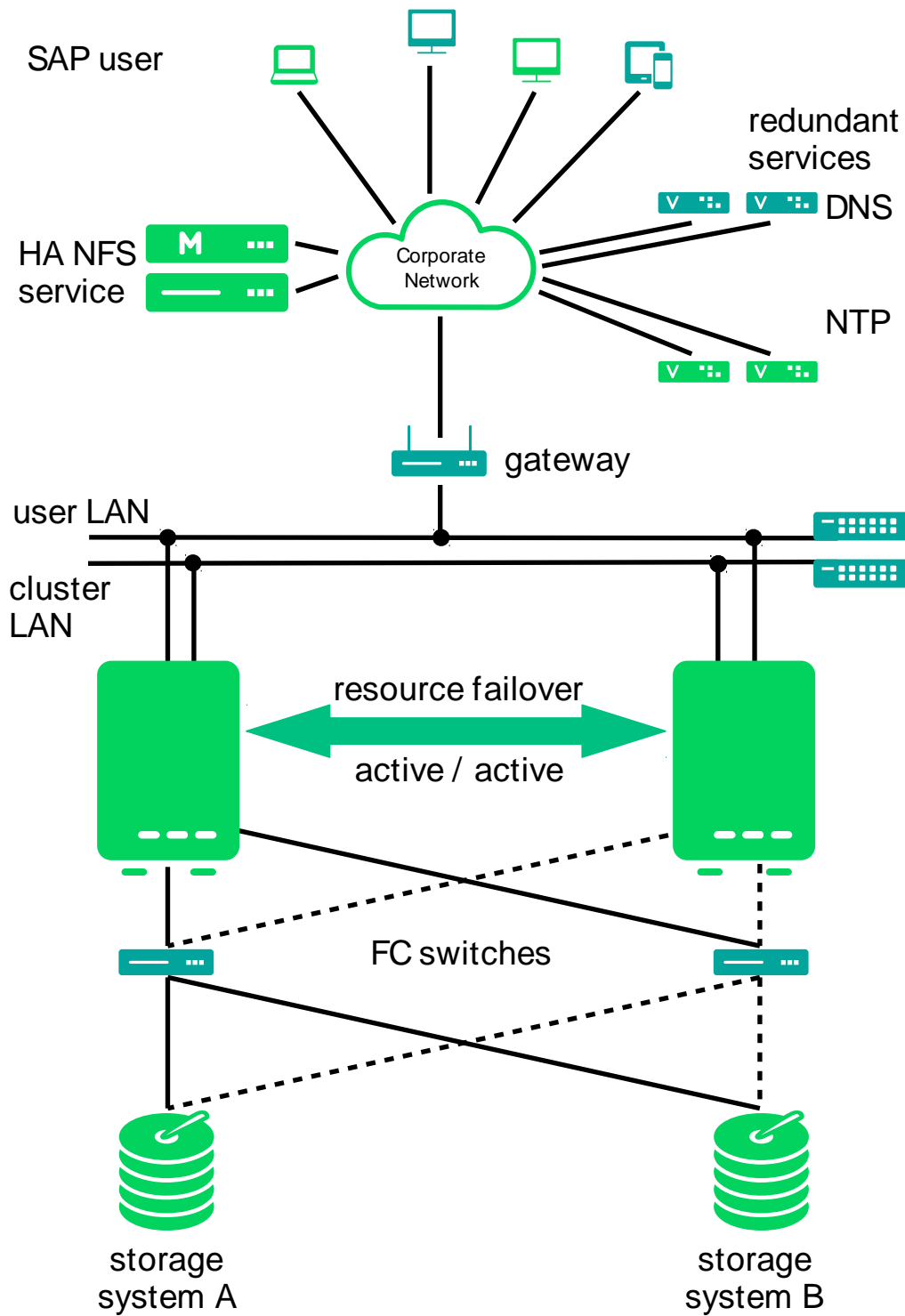
FIGURE 4.1: GENERAL ARCHITECTURE
